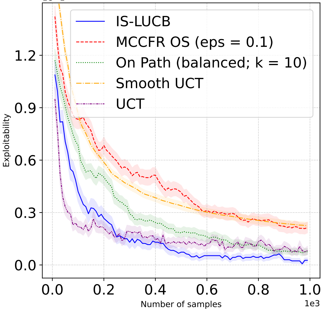
1e-1 Kuhn Poker, Best Algorithms, Player o
